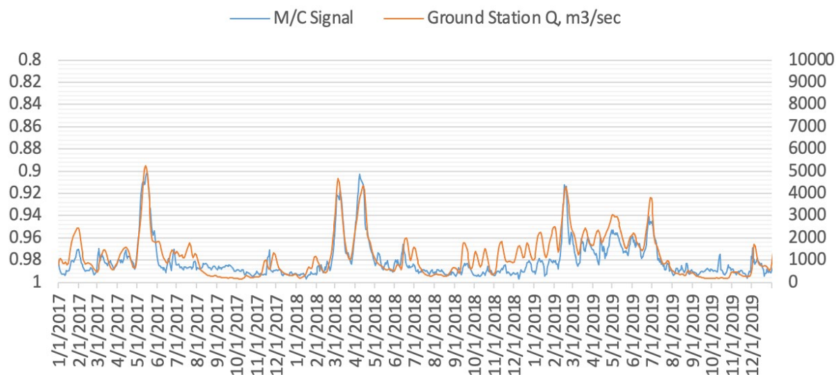
Figure 2, Sensor data (M/C ratio, left axis) directly compared to co-located USGS gauging station data (right axis) for a portion of the SGR 91 record, Wabash River, U.S. This is a 200 m wide meandering river.
